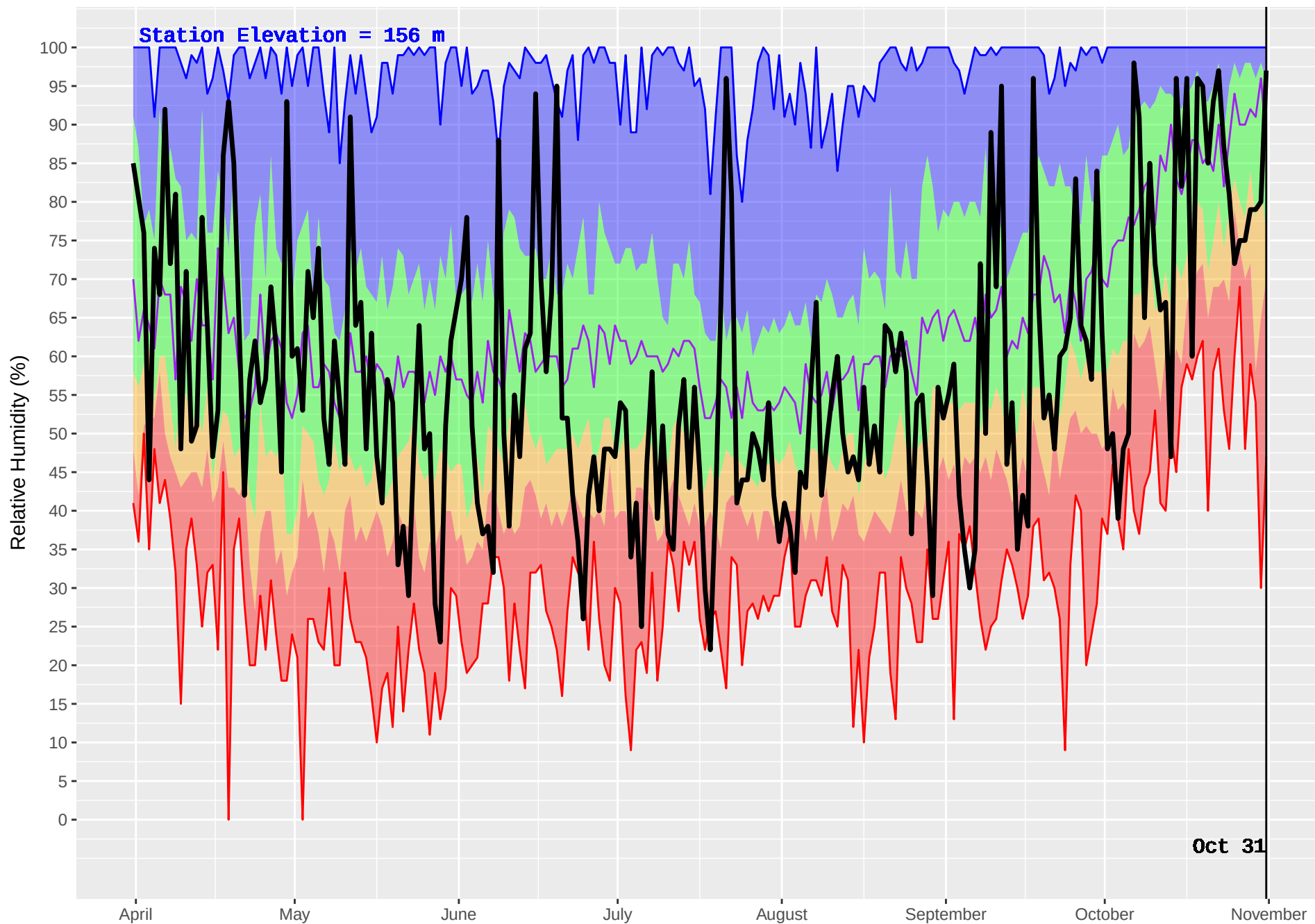
WOSS CAMP (21) : Historical (1970–2016) and Current (2017) Noon Relative Humidity
