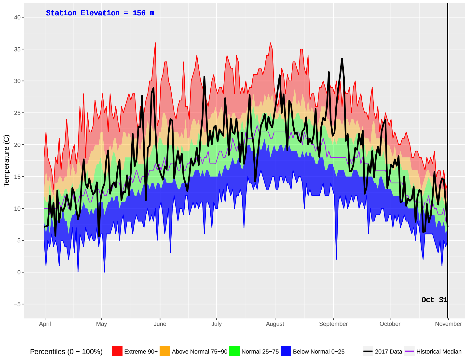
WOSS CAMP (21) : Historical (1970–2016) and Current (2017) Noon Temperature
