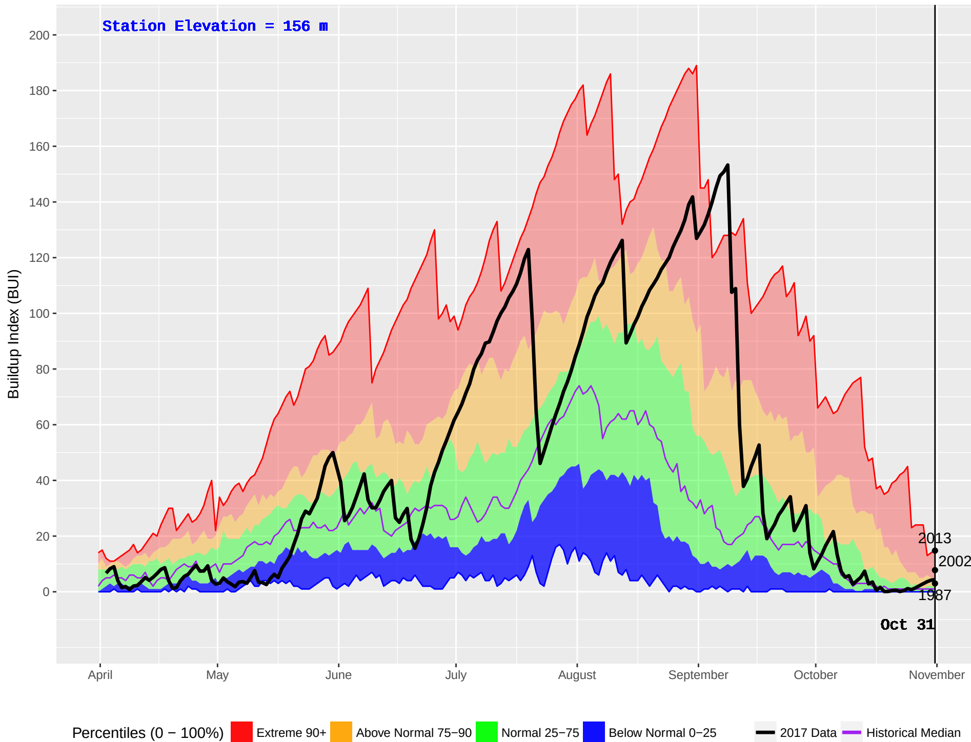
WOSS CAMP (21) : Historical (1970–2016) and Current (2017) Noon Buildup Index (BUI)
